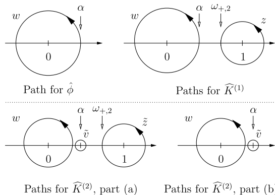
Fig. 4 Steep descents for the different terms in the kernel. The path w passes either through \alpha or at distance \varepsilon T^{-1/2} from it
