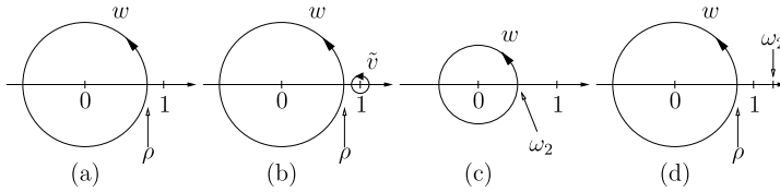
Fig. 7 Steep descent paths used for the different terms, with \rho = 1 - \varepsilon(t/2)^{-1/2} . (a) Is for term (1); (b) For term (2) and (3a); (c) For term (3b) in case \tau_1 < \tau_2 ; (d) For term (3b) in case \tau_1 > \tau_2
