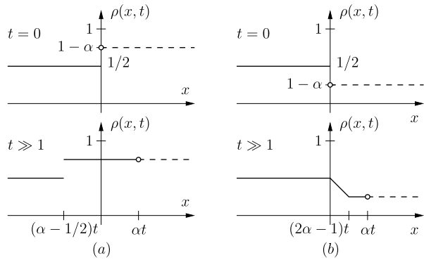
Fig. 1 Particles' density for large t : (a) for 0 < \alpha < 1/2 , (b) for 1/2 < \alpha < 1 . The big dot is the position of the right-most slow particle
