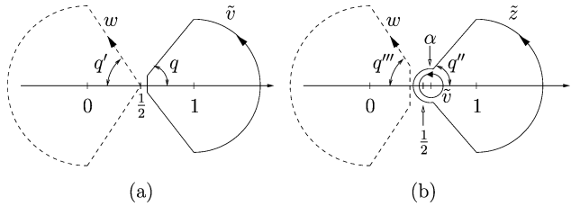
Fig. 6 Steep descents for (a) \widehat{K}^{(1)} and (b) \widehat{K}^{(2)} . They satisfies \pi/4 < q < q' < \pi/2 , \pi/4 < q'' < q''' < \pi/2 and the local modifications around the critical point at 1/2 are all only on the T^{-1/3} scale
